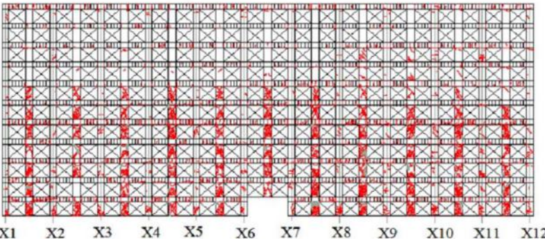
(b) Damaged frames
