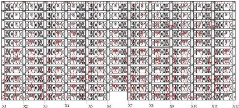
(a) Non-structural walls failed in shear
