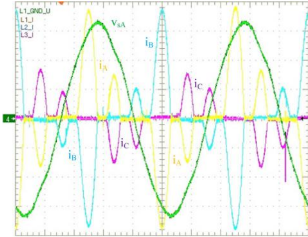
Fig. 20. Mains input phase currents (20 A/div) and voltage (100 V/div) for pulsed operation.
