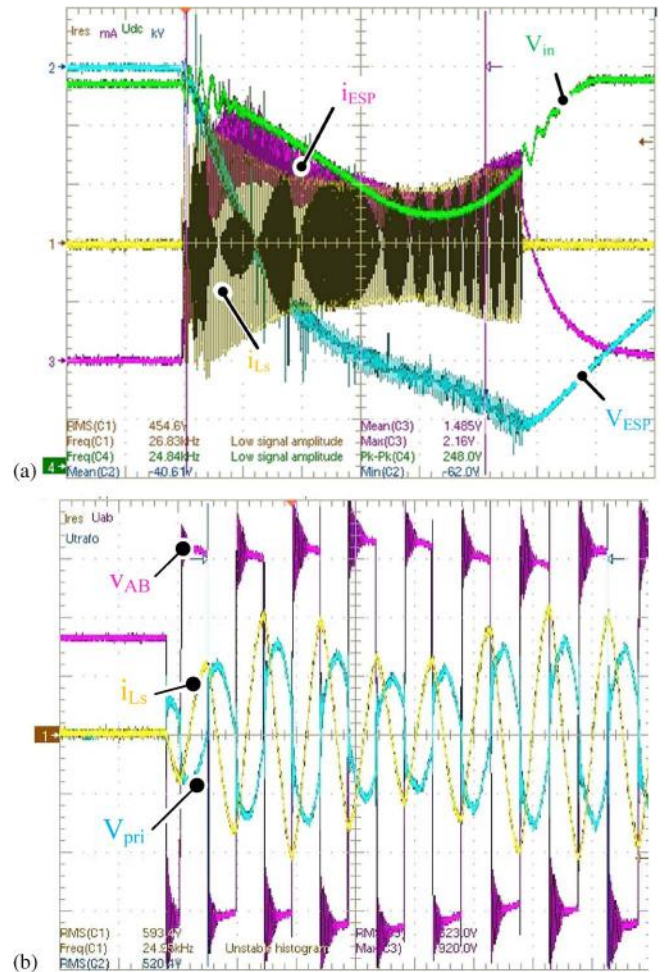
Fig. 19. Pulsed operation main waveforms. (a) Resonant tank current i_{Ls} (100 A/div); output voltage V_{ESP} or V_o (10 kV/div); current i_{ESP} (250 mA/div); and bus-bar voltage V_{in} (100 V/div). (b) Resonant tank current i_{Ls} (100 A/div); full-bridge output voltage V_{AB} (200 V/div); and transformer primary voltage V_{pri} (500 V/div). Signal V_{pri} is inverted.
