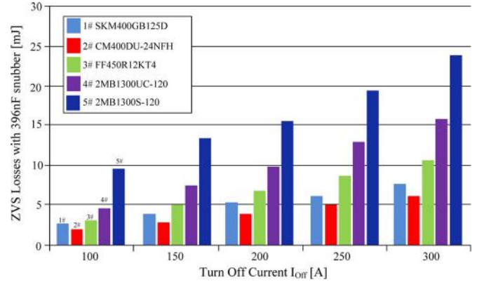
Fig. 8. ZVS turn off measurement results, T_J = 125^\circ\text{C} and C_{Snb} = 396\text{ nF} .
