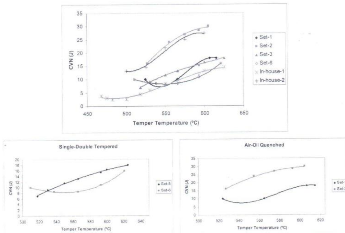
Fig. 1. Variation of CVN for H13 samples, single and double tempered to different tempering temperatures; air and oil quenched
