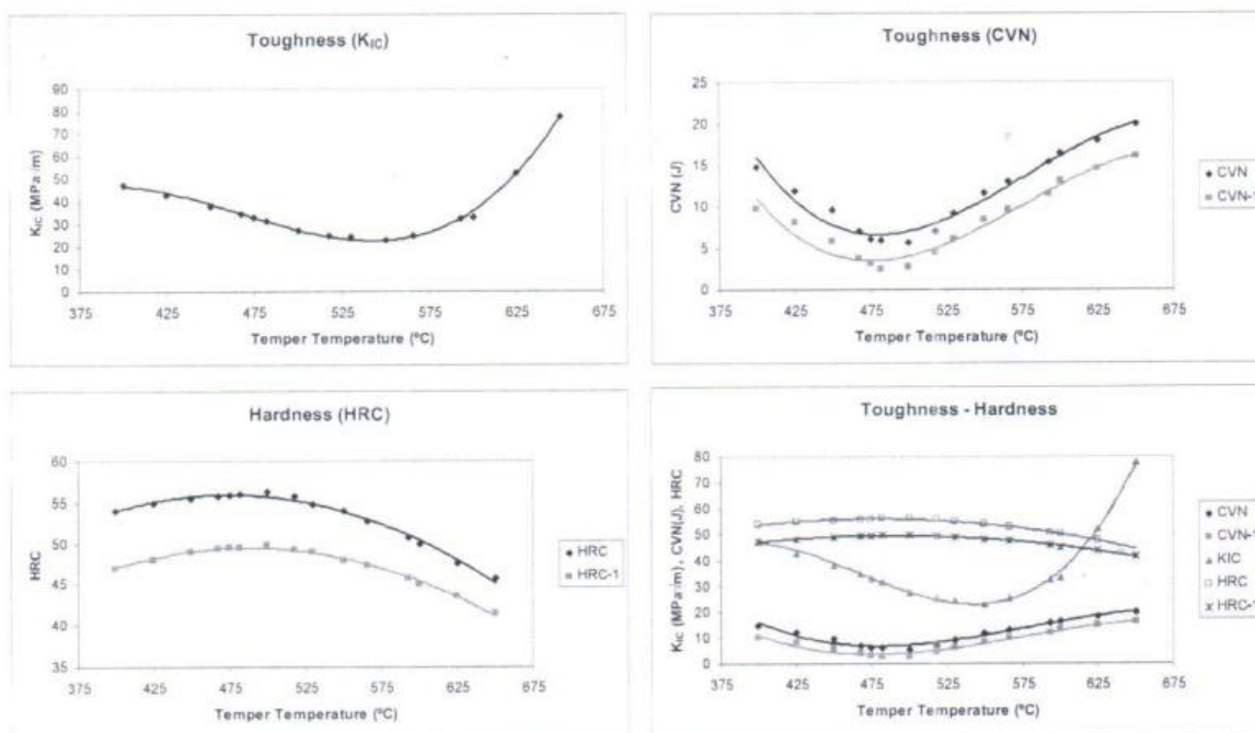
Fig. 3. Variation of fracture toughness, impact energy, and hardness; H13 samples single tempered to different tempering temperatures
