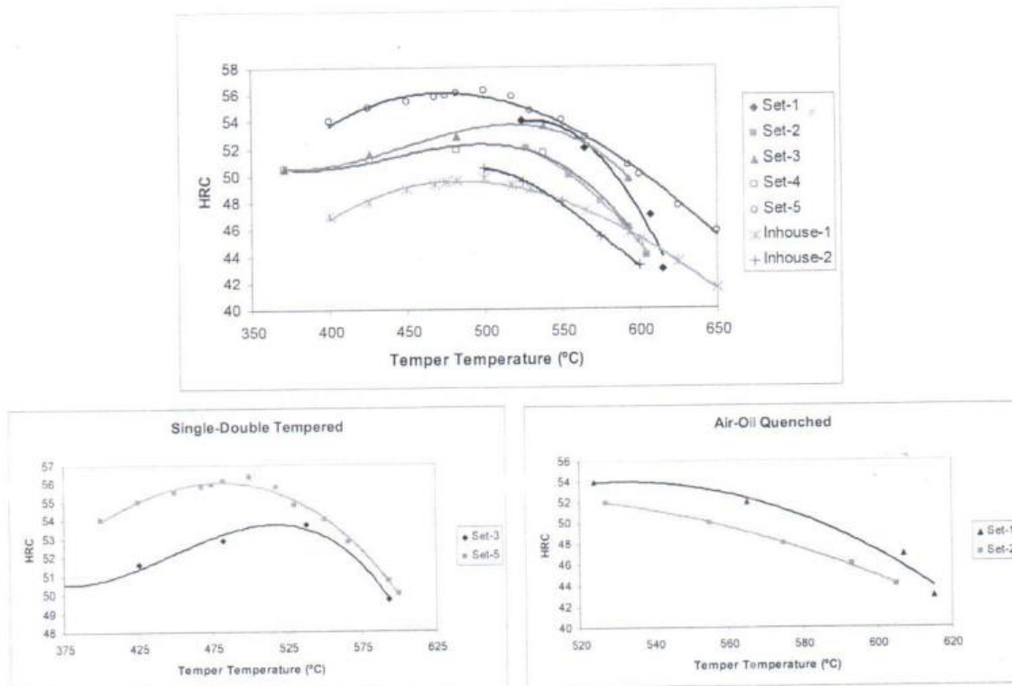
Fig. 2. Variation of HRC for H13 samples, single and double tempered to different tempering temperatures; air and oil quenched
