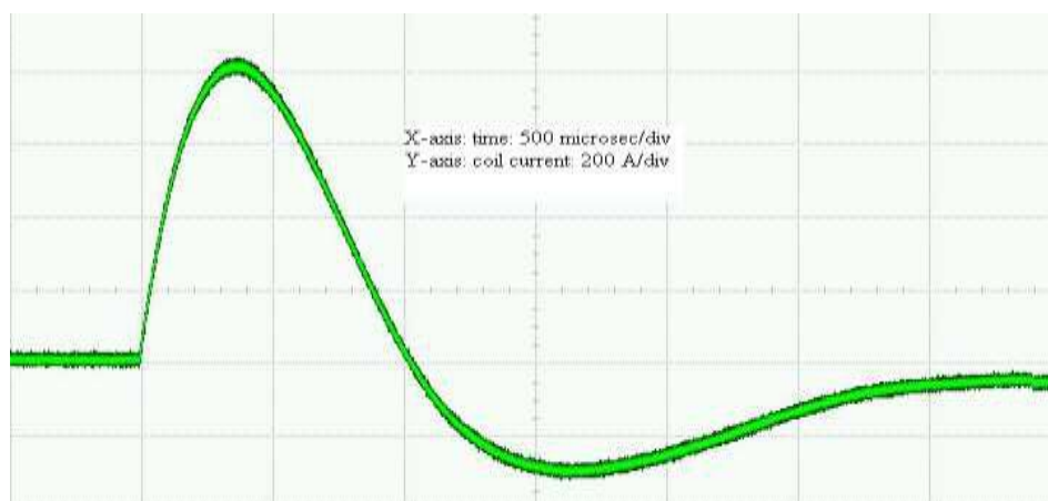
Fig.8. Actual waveform of coil current
