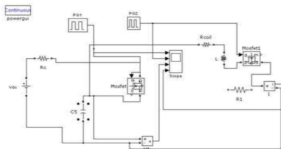
Fig.6. MATLAB simulation of coilgun circuit
