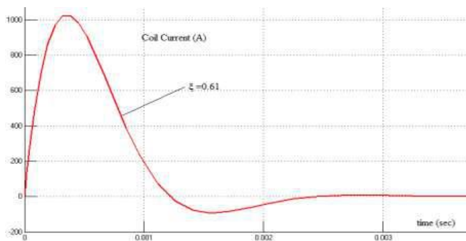
Fig.7. Simulated current waveform
