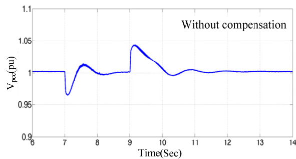
Fig. 4 V_{pcu} of the system without any compensation
