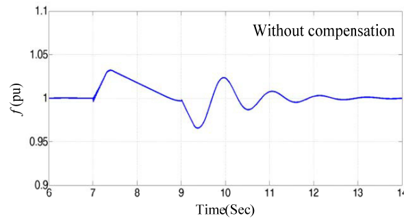
Fig. 5 Frequency of the system without any compensation
