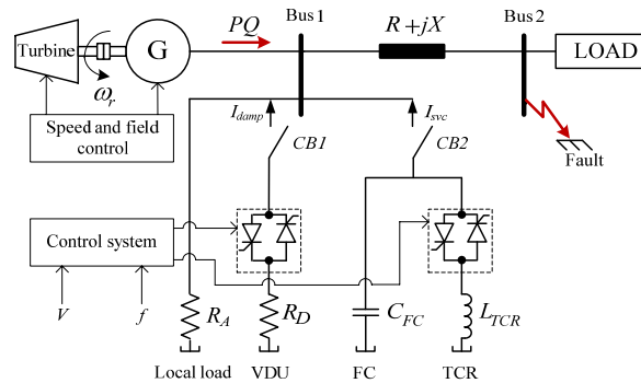
Fig. 1. System configuration
